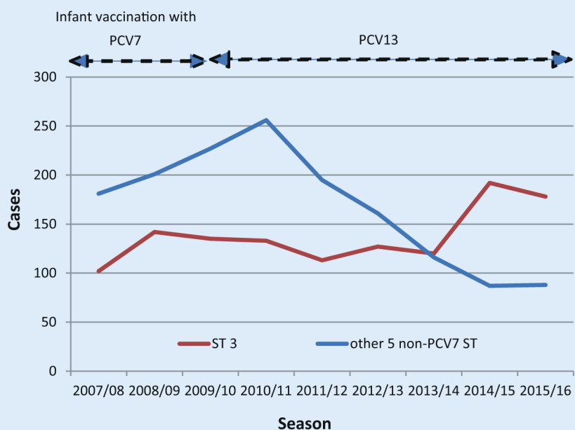
Fig. 4 ▲ IPD cases in people aged ≥60 years, caused by the 6 serotypes (1, 3, 5, 6A, 7F, 19A) included in PCV13 but not PCV7
