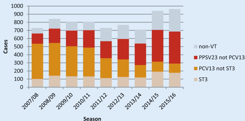
Fig. 3 ▲ Serotype distribution of the IPD cases recorded on PneumoWeb in seniors 60 years and over, absolute case numbers
