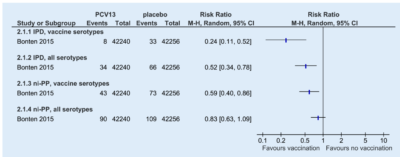
Fig. 7 ▲ Efficacy of PCV13 against invasive pneumococcal diseases (IPD) and non-invasive pneumococcal pneumonia (ni-PP), CAPITA RCT, modified intention-to-treat analysis This graph was created using the Review Manager software. In some cases, the boundaries of the confidence intervals (CI) deviate slightly (by 0.01 to 0.02) from the figures in the publication, where a different statistical procedure was used to calculate the CI, and in some cases a 95.2 % CI was given
